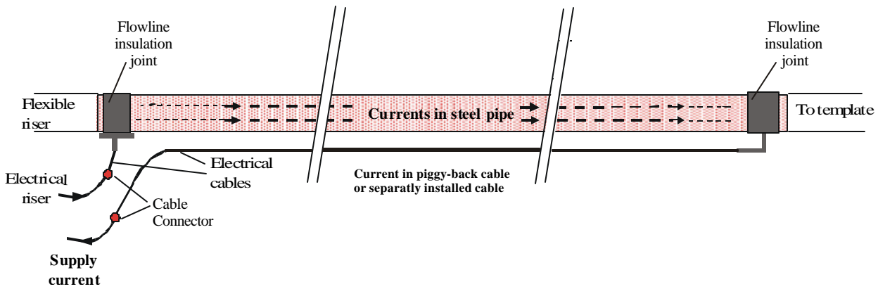
Figure 4 Circuit with cable return
