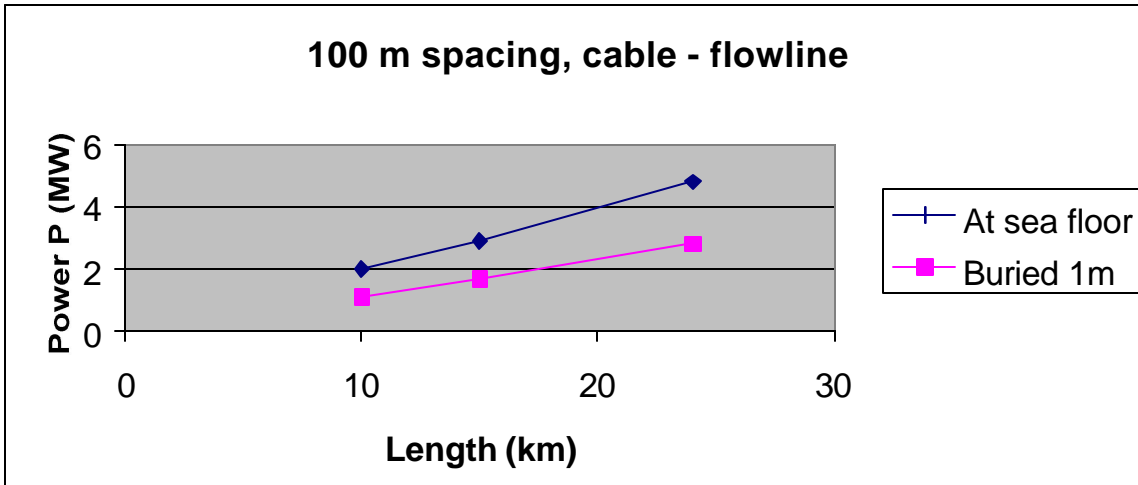
Figure 10-Power as function of length, buried and not buried
