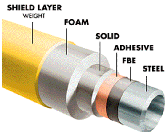
Figure 1-Flowline with polypropylene multi-layer insulation
