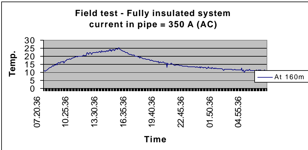
Figure 12-The temperature is measured at several positions along the flowline, on the inner diameter of the pipe. This diagram shows the temperature 160 m from land, during one heating cycle.
