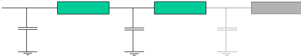
Figure 6-Equivalent p circuit
