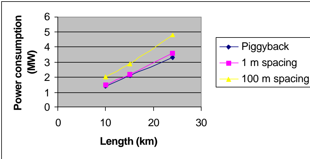
Figure 8-Power consumption as a function of length
