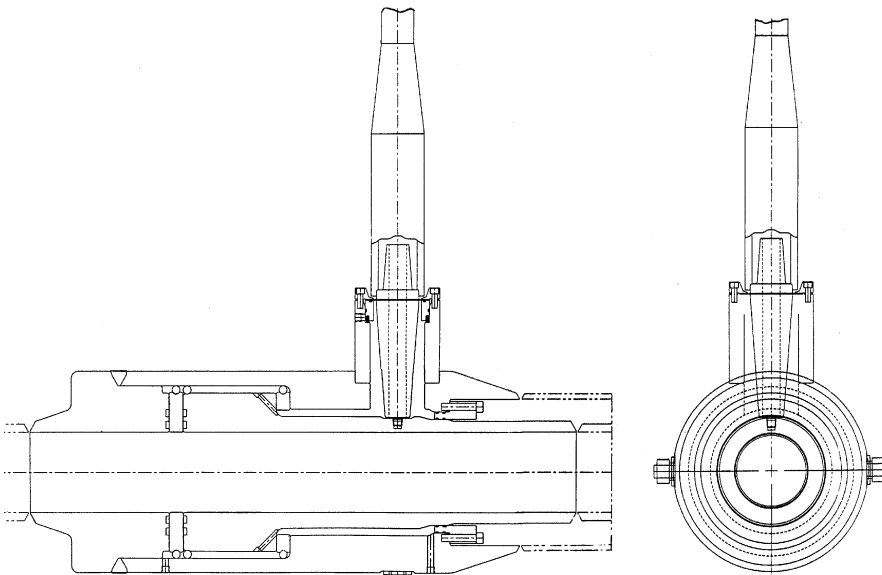
Figure 3 Flowline insulating joint
