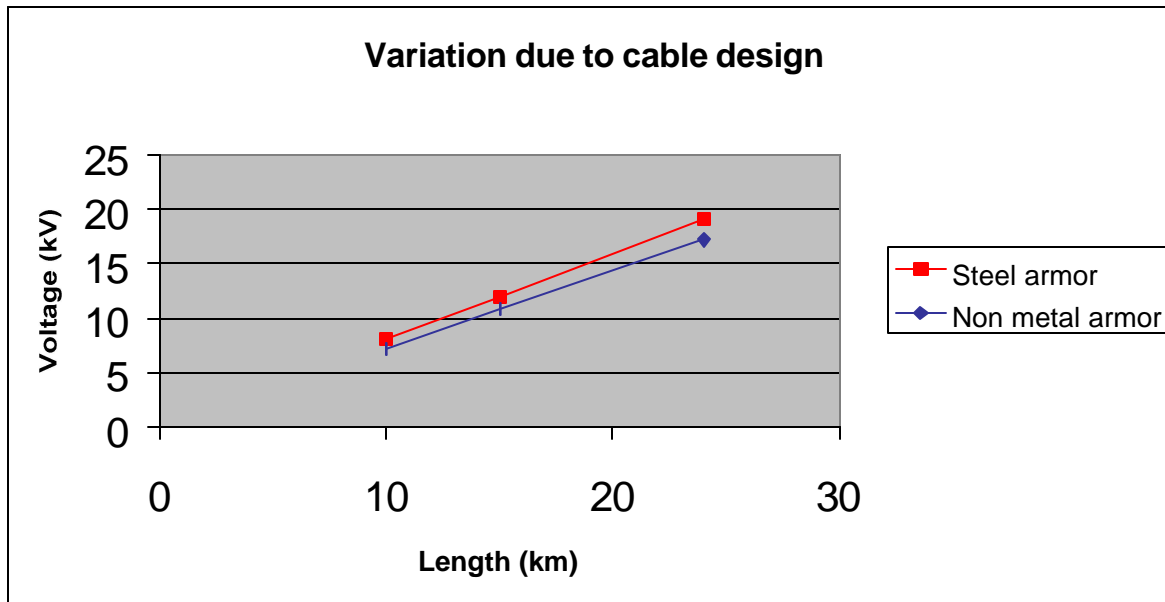
Figure 9-Voltage variation due to cable design, 100m spacing
