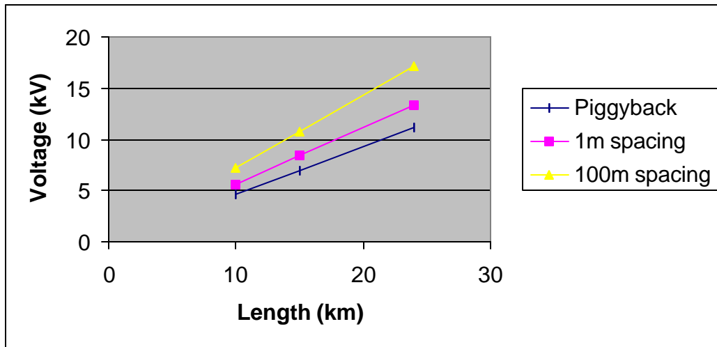
Figure 7 Voltage as function of length
