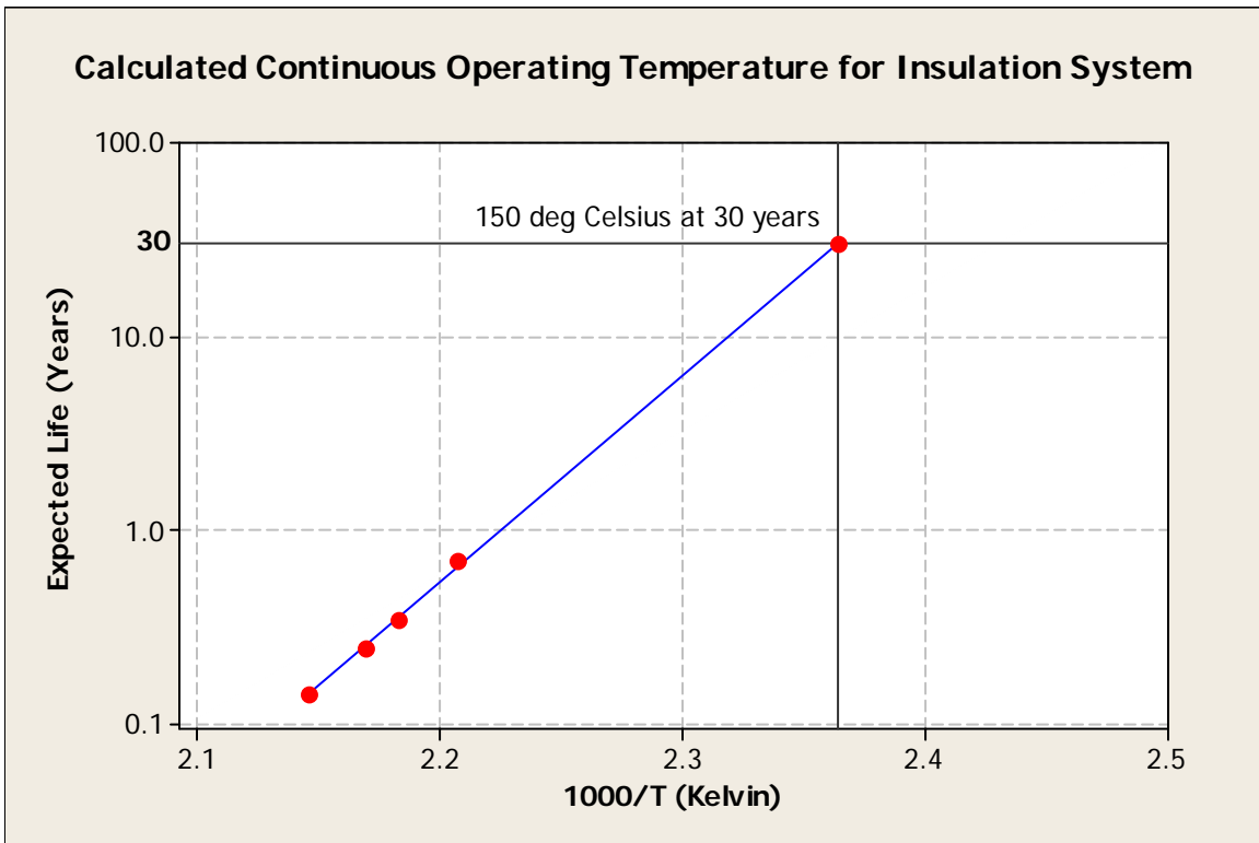
FIGURE 5 - Calculated Thermal Life (CCOT) For Insulation System
