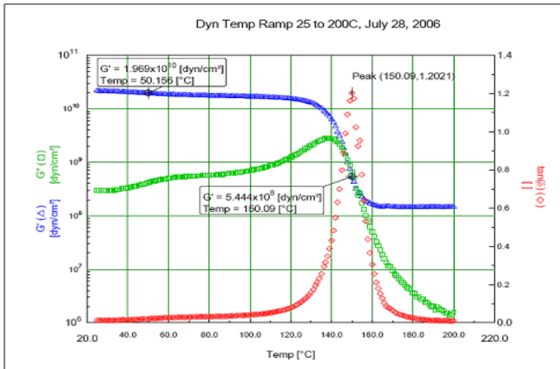
FIGURE 2 - DMA Test Results for Epoxy Coating
