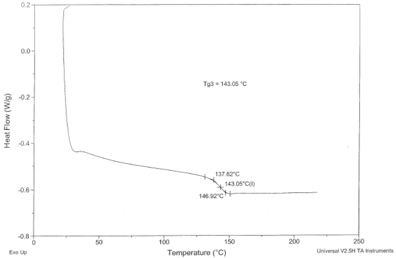
FIGURE 3 - DSC Scan for Glass Transition Temperature of FBE
